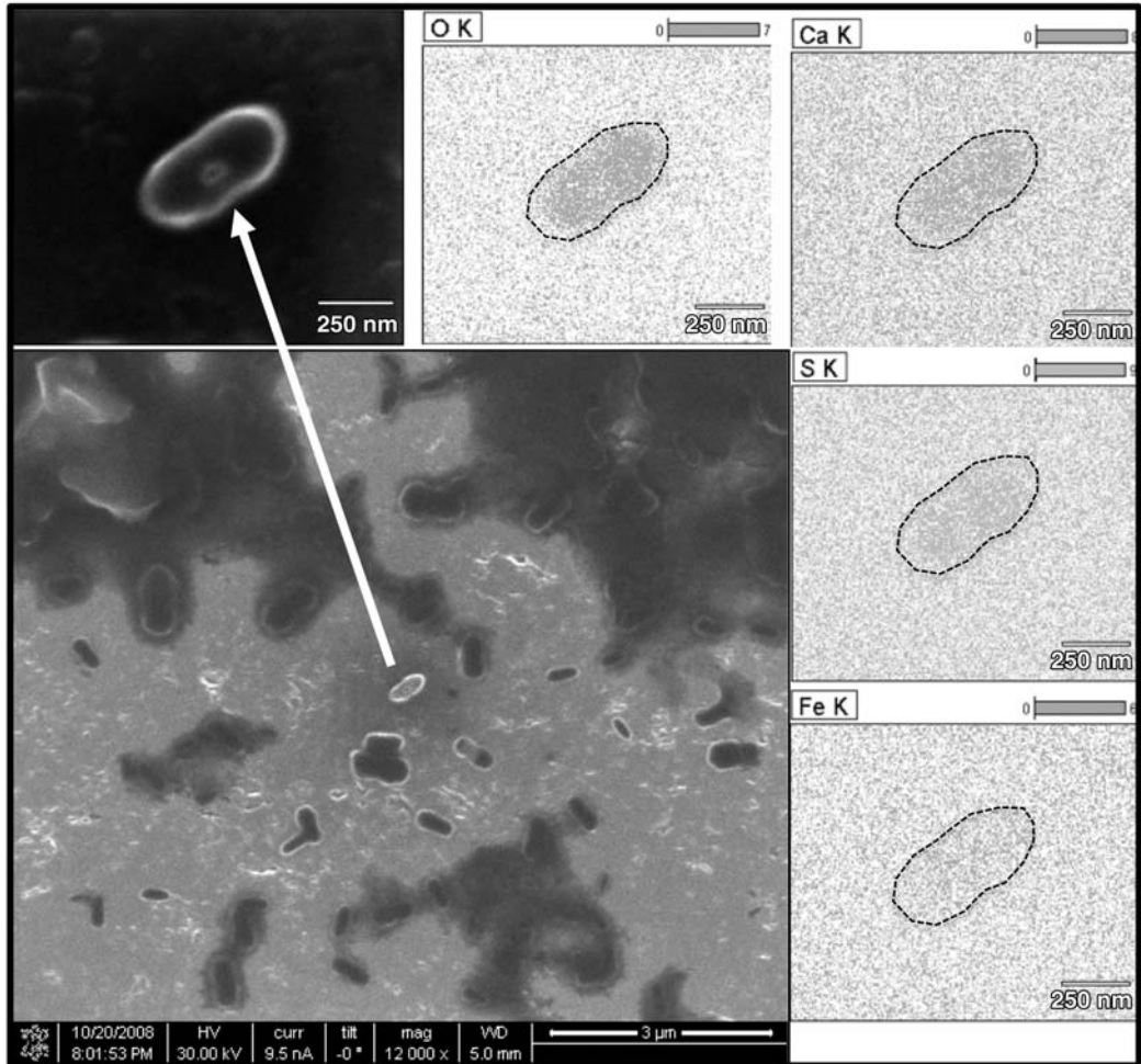
FIG. 11. SEM and energy dispersive X-ray maps showing microbe-shaped bodies, in the OMT Blue clay, which concentrate O, Ca, S and Fe. These are interpreted as environmental microbes which metabolize and concentrate \text{Fe}^{2+} .
