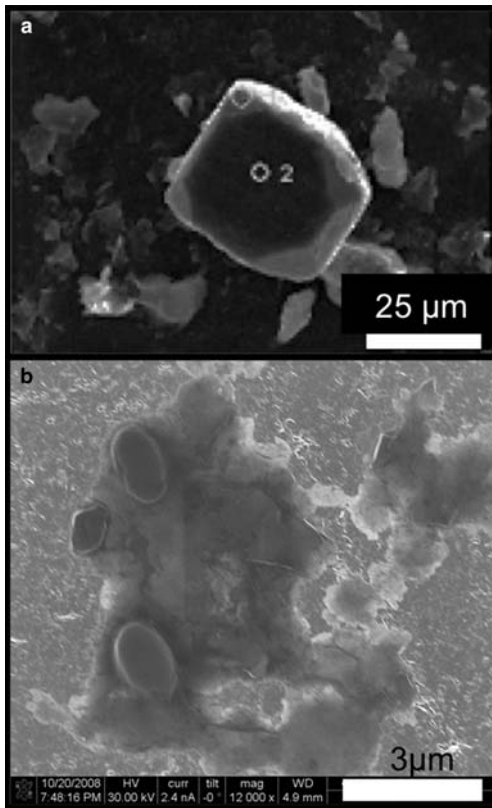
FIG. 10. Pyrite morphologies in the OMT Blue clay alteration assemblage. (a) Crystalline pyrite is >10\ \mu\text{m} across, whereas (b) <1\ \mu\text{m} Fe-S-bearing spheres are abundant in the clay matrix (Williams et al. , 2011).
