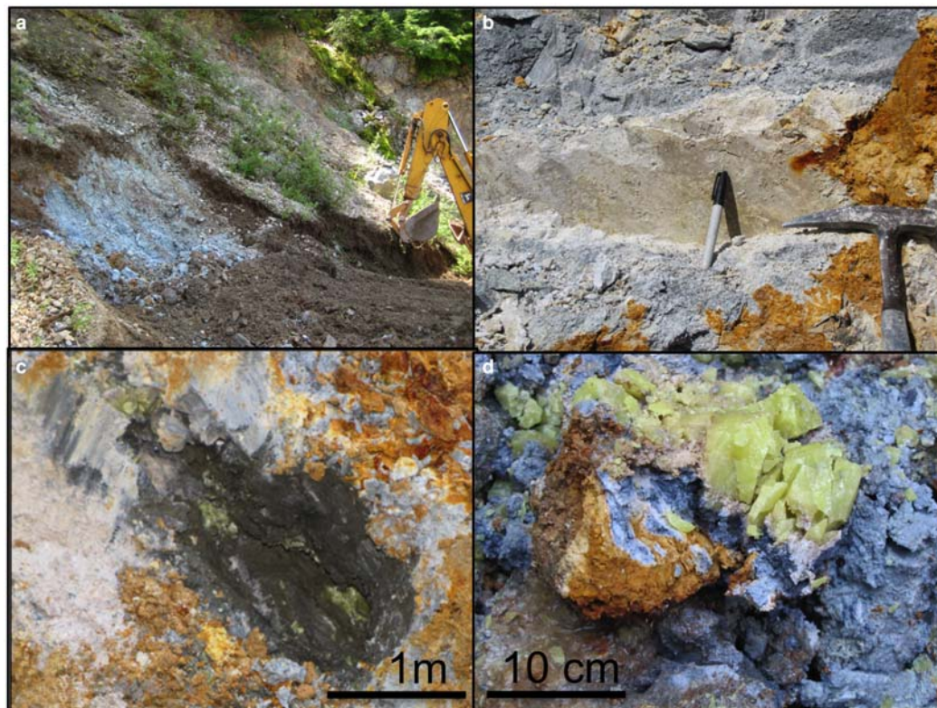
FIG. 7. Clay alteration assemblages studied in the OMT deposit. (a) Blue clay, (b) White clay in fault zones, (c) Black clay rich in pyrite, (d) Red oxidized surface clay found at all locations and elemental sulfur from the Sulfur mine location (photos by K.D. Morrison, 2015).
