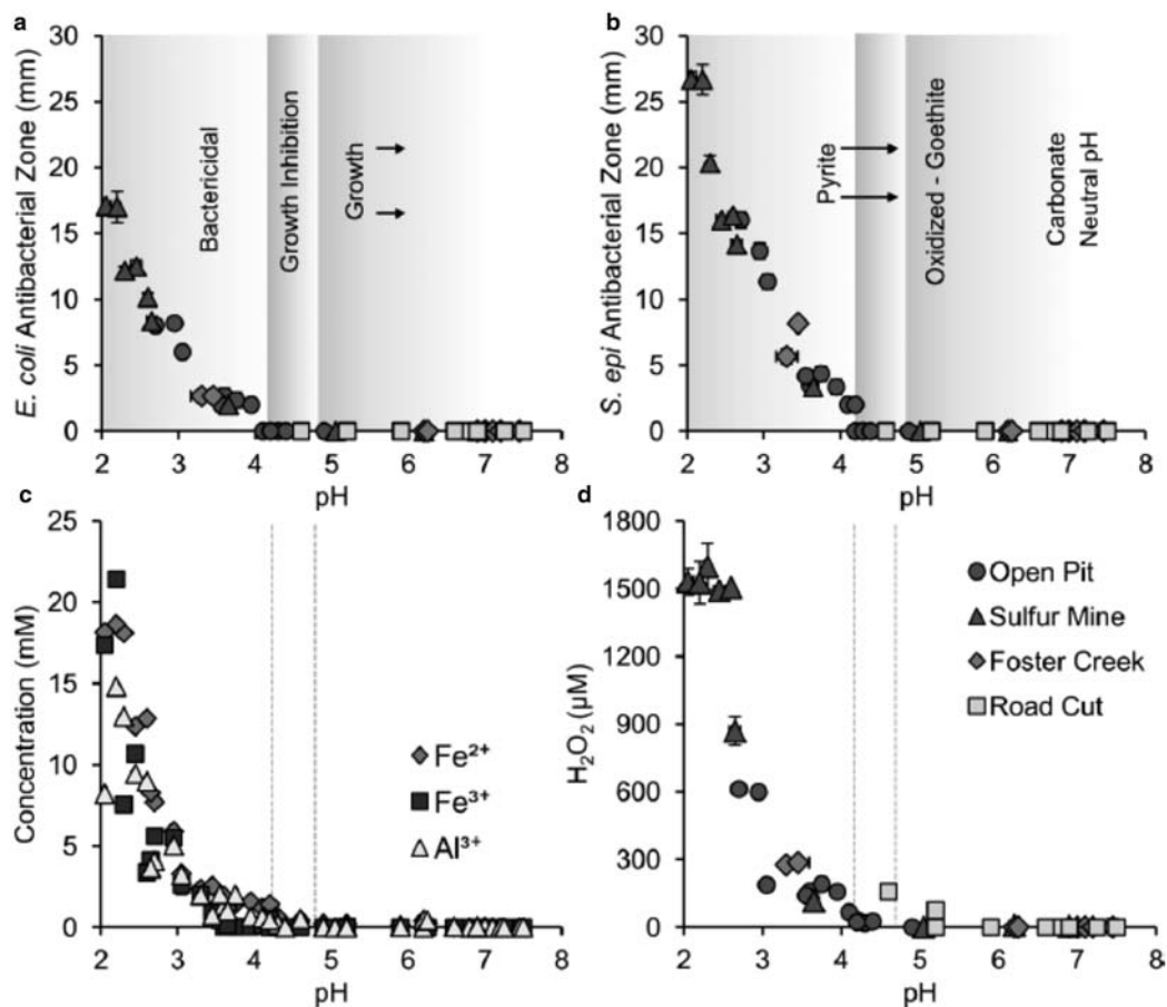
FIG. 13. Trends with pH in antibacterial effectiveness across the OMT deposit, indicated by zones of inhibition (mm) from clay suspensions (100 mg/mL): (a) Gram-negative E. coli ; (b) Gram-positive S. epidermidis ; (c) major metals in solution; (d) hydrogen peroxide (from Morrison et al. , 2016; open access).
