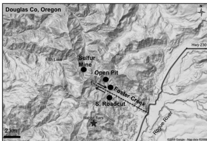
FIG. 6. Field area of the Oregon Mineral Technologies deposit and major sites sampled.
