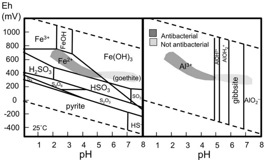
FIG. 14. Eh-pH stability plots at 25°C for aqueous: (a) Fe-S-O (modified from Morrison, 2015) and (b) Al-O (data from Takeno, 2005) showing the range of antibacterial and non-antibacterial clay suspensions from the OMT alteration assemblages.
