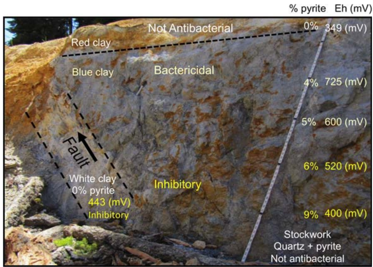
FIG. 12. Cross section sampled through the OMT Blue clay in the Open Pit reveals that the antibacterial effectiveness decreases with depth as the oxidation state of the hydrated clay decreases. The pyrite content increases with depth, but is negatively correlated with bactericide. Oxidation state is the dominant control on the antibacterial process.
