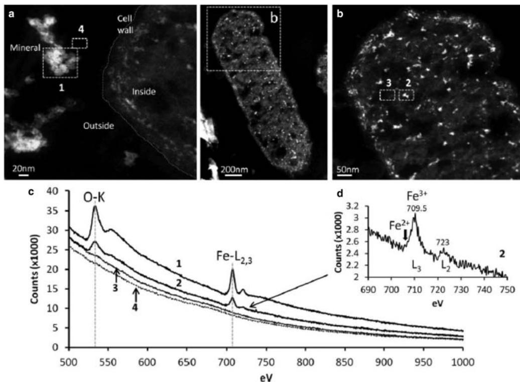
FIG. 18. Electron energy loss study of the opaque precipitates observed in E. coli reacted for 24 h with OMT leachate (from Morrison et al. , 2014): (a) areas 1 and 4 compare mineral to no mineral; (b) close-up of electron-dense area 2, compared to 3 background; (c) EEL spectra for areas 1–4; and (d) close up of energy spectra indicating Fe 3+ precipitates.
