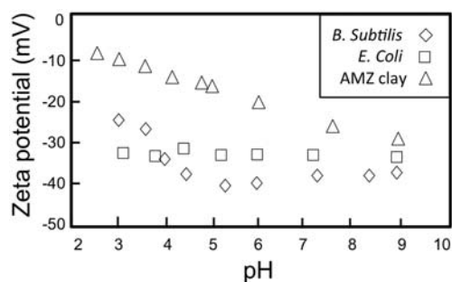
FIG. 19. Zeta potential of two model bacterial pathogens compared to the AMZ clay suspension in DIW (equilibrated for 24 h).
