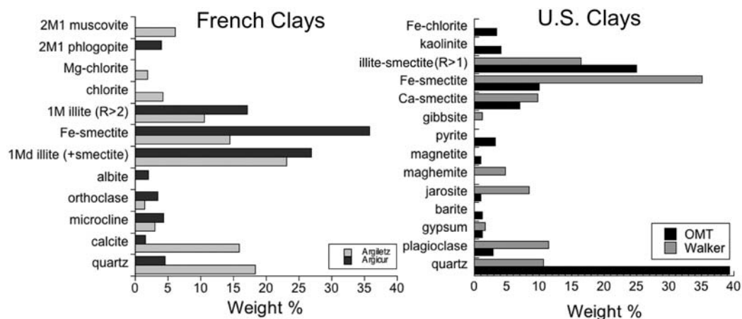
FIG. 4. Mineralogical comparisons of the two French clays and two US antibacterial clays. The mineralogy was determined by X-ray diffraction (Cu-K \alpha ) on bulk powders, using RockJock (Eberl, 2003) for quantification.
