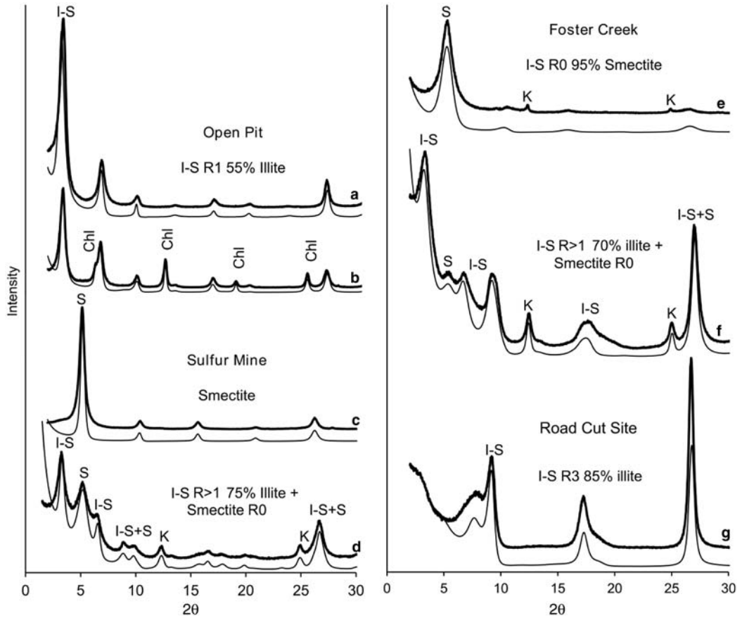
FIG. 9. XRD patterns of oriented, ethylene glycol-saturated <2 \mu\text{m} size fraction separates from (a) Open Pit Blue clay, (b) Open Pit perimeter, (c) Sulfur Mine White clay, (d) Sulfur mine Blue clay, (e) Foster Creek White clay, (f) Foster Creek Blue clay, (g) Roadcut Blue clay (Sample locations in Fig. 6; data from Morrison, 2015).
