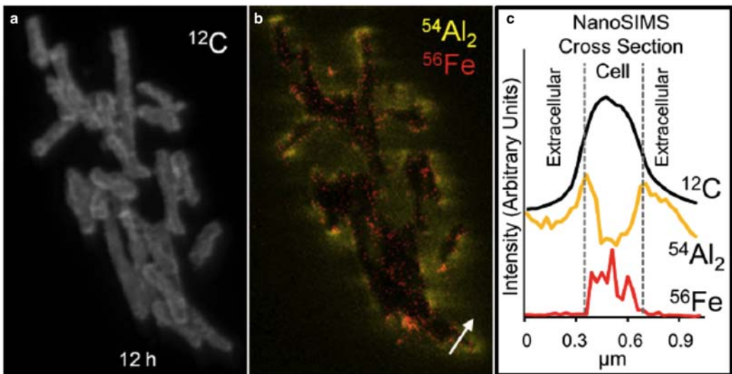
FIG. 17. NanoSIMS showing: (a) a cluster of E. coli treated with OMT leachate; (b) Al (yellow) and Fe (red) distributions in the E. coli ; (c) cross section across a single cell (white arrow in b) showing elevated Al on cell membranes and intracellular Fe (modified from Morrison et al. , 2016).
