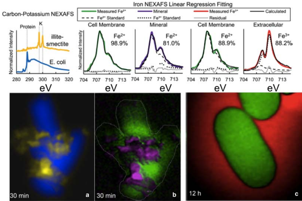
FIG. 16. Near-edge X-ray absorption fine structure mapping of Fe in OMT Blue clay suspensions with E. coli (modified from Morrison et al. , 2016). (a) I-S (yellow) is indicated by K content on E. coli (blue) after 30 min; (b) Fe 2+ -dominant clays (purple) on Fe 2+ -enriched cell membranes (green); (c) Fe 2+ is attracted preferentially to cells (green) after 12 h, leaving Fe 3+ -enriched fluid (red).
